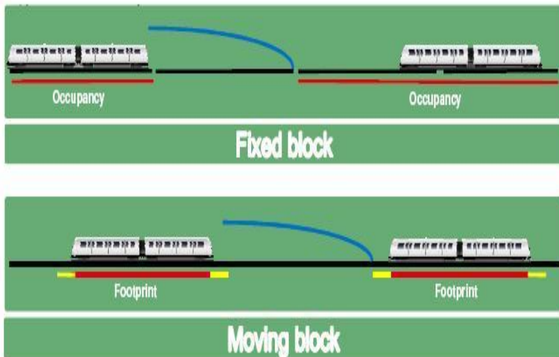
Fig 1: CBTC Railway System
